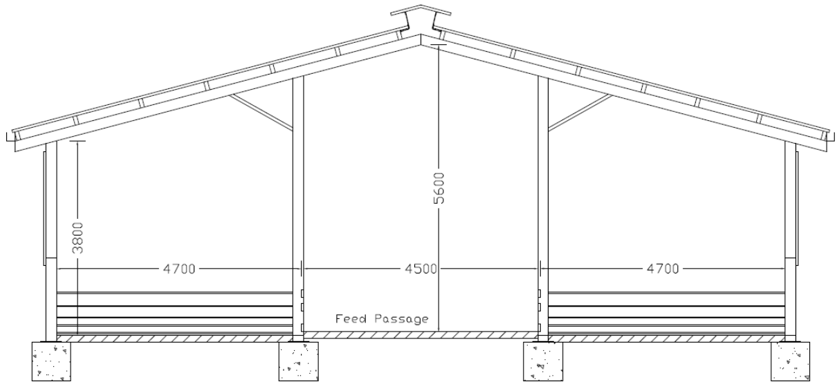
Section BB - straw-bedded sheep house
