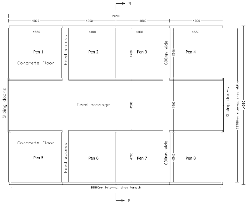
Plan view - 4 bay straw-bedded sheep house
